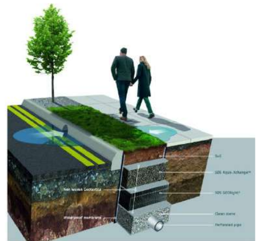
Typical section for attenuation tank installation
