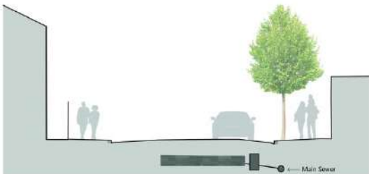
Section B-B' Existing pavement | Permeable paving rainwater collection system and attenuation tank | Existing pavement
